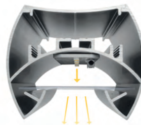
DIRECT lighting system
