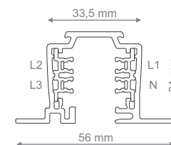
LU TRACK recessed
